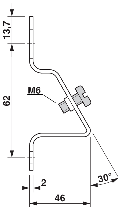
Dimensional drawing
