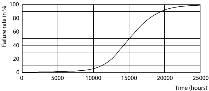
Life Expectancy Diagram - CorePro LEDcapsuleLV 0.9-10W G4 830
