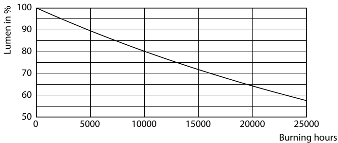
Lumen Maintenance Diagram - CorePro LEDcapsuleLV 0.9-10W G4 830
