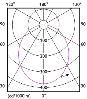
Light Distribution Diagram - MAS LED spot VLE D 650lm GU10 930 120D
